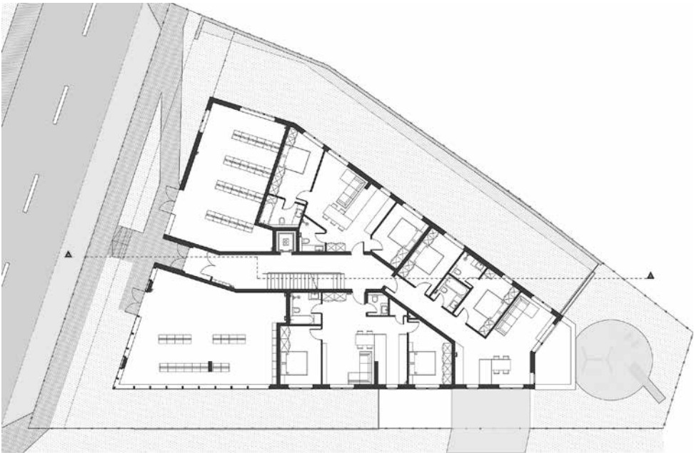
Plan parter
